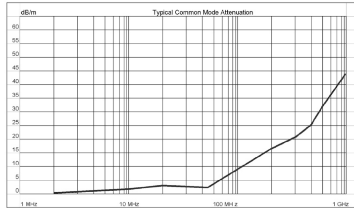
Ferrite Coated Low Pass Squib Filter Wire LP/LIMY 2 x 0.25 mm 2
